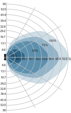
Wall mounting pattern (Unit: ft) Suggested installation height: 3.2 - 5.9 ft
