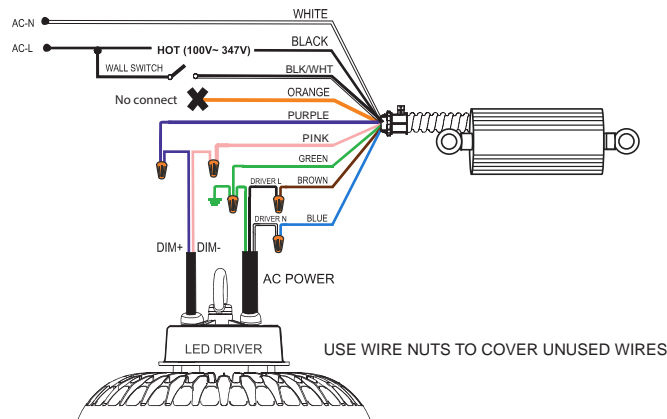
FIG A. without dimmer and sensor
