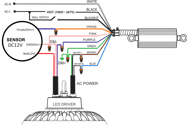
FIG C. with DC sensor
