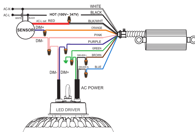
FIG D. with AC sensor
