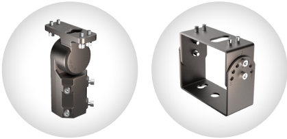
Pre-Installed Slipfit Knuckle Mount Trunnion Mount
