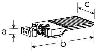
Trunnion Arm Mount
