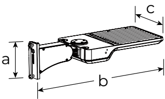
Adjustable Straight Arm Mount
